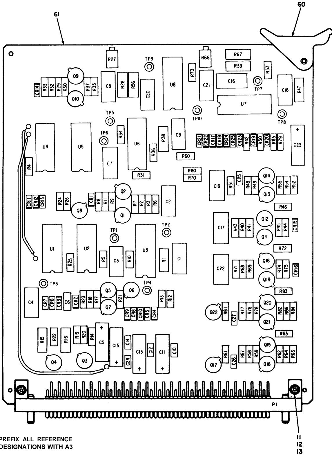
Figure 5. Circuit Card Assembly, Mode 4 Interface and Trigger Generator (A3) (Sheet 1 of 2)
