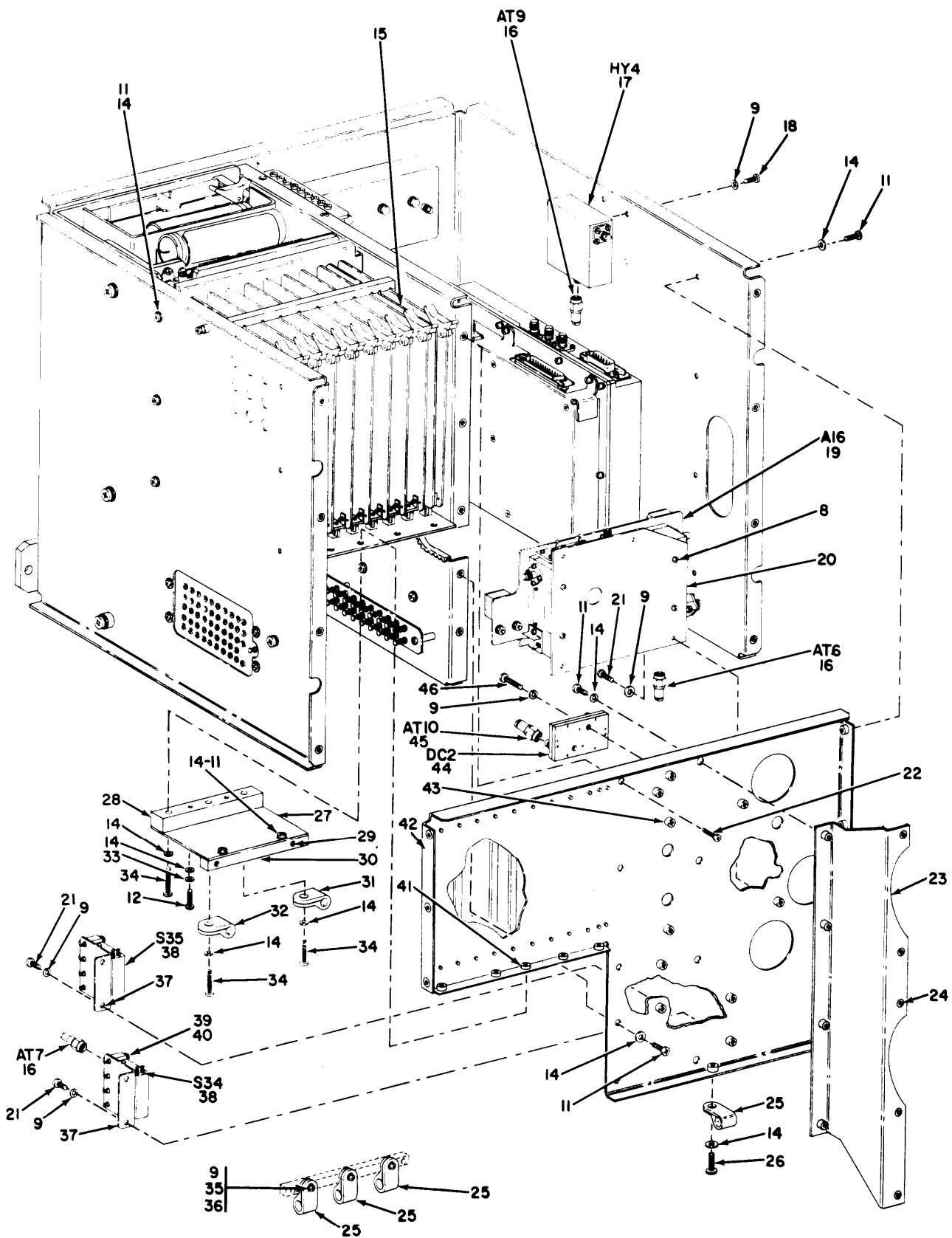
Figure 2. Test Set, Radar TS-3394A/TPM-25 (Sheet 2 of 4)
