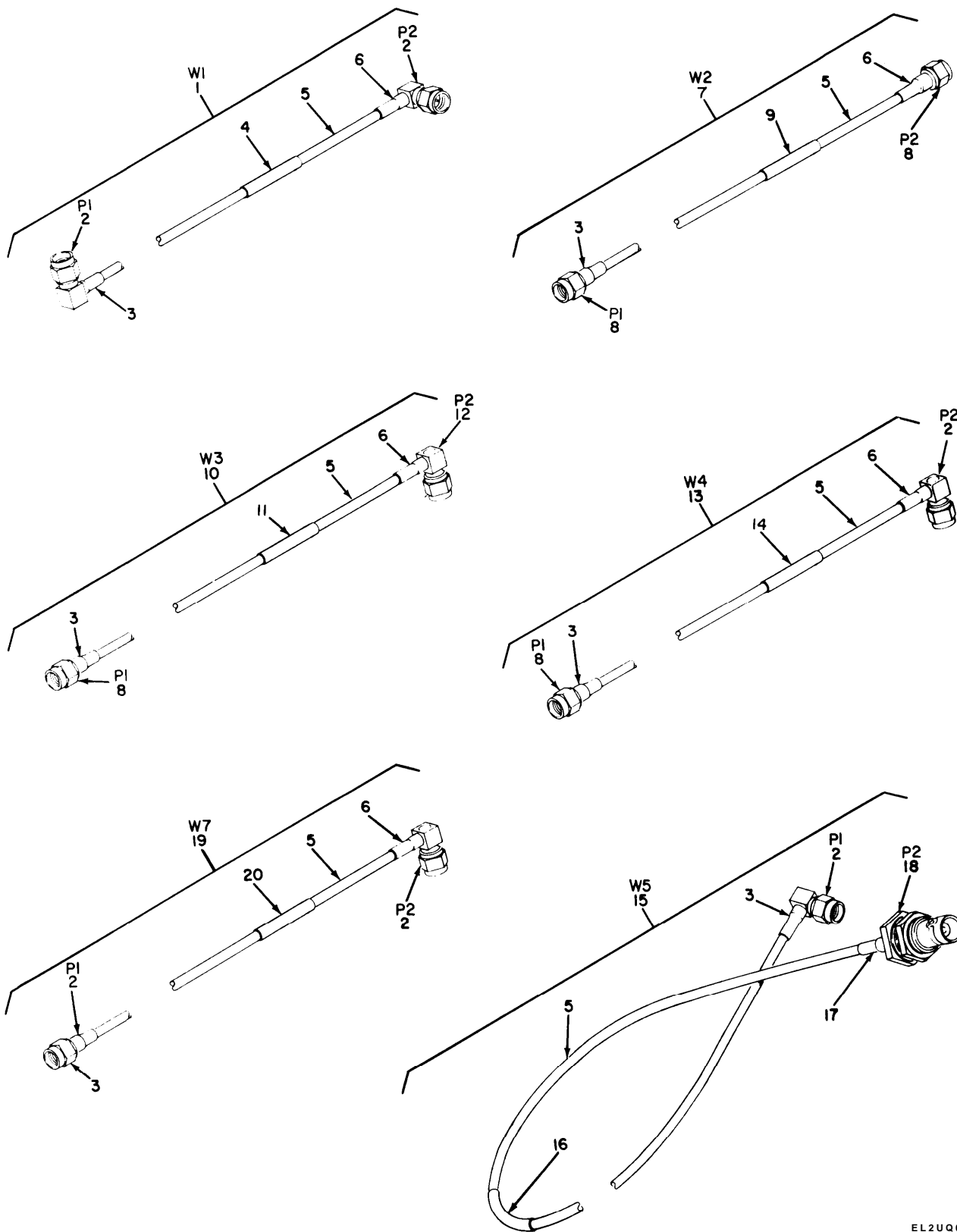
Figure 27. Cable Assemblies, RF (152177-- and 151178--) (Sheet 1 of 4)
