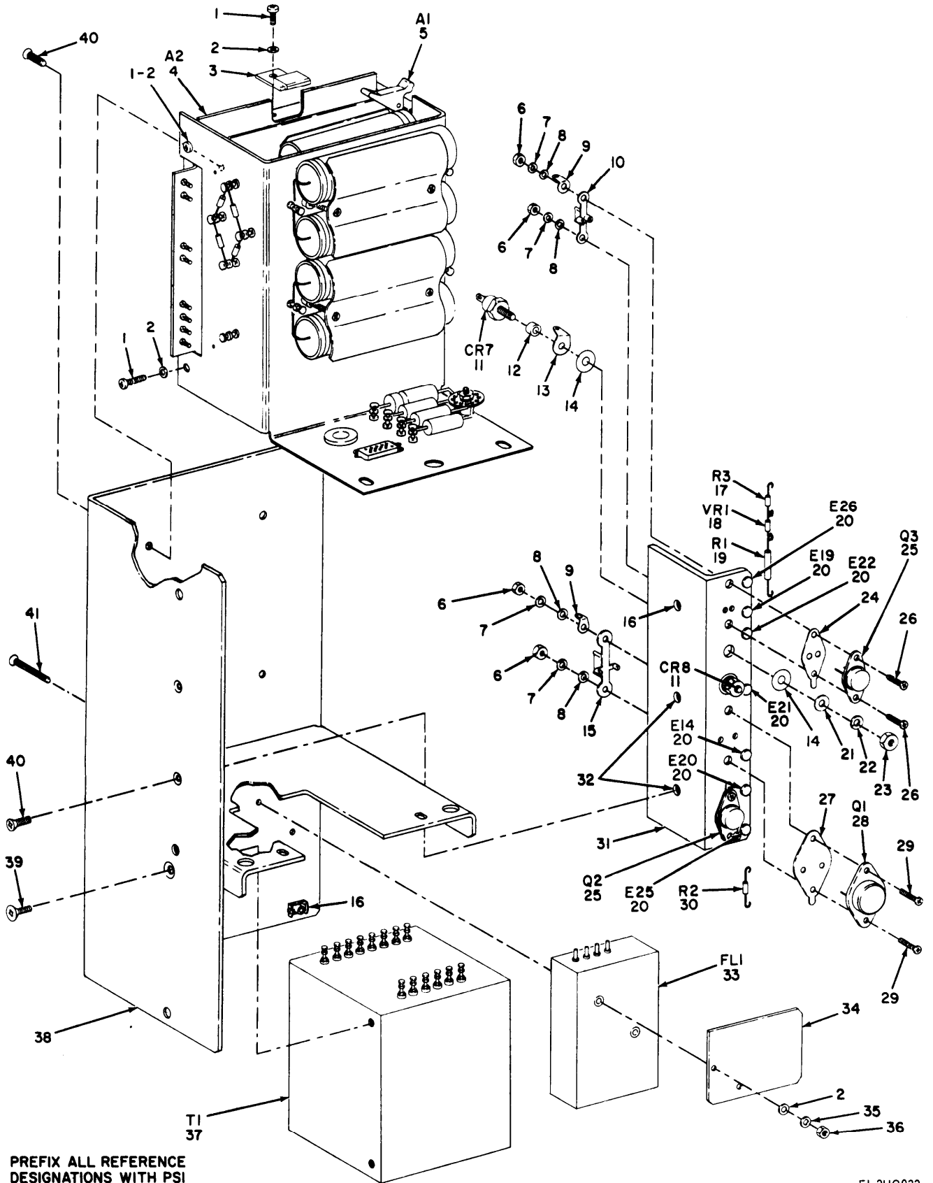
Figure 23. Power Supply Assembly (PS1) (Sheet 1 of 2)
