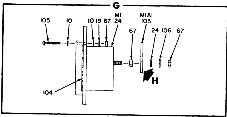
Figure 26. Control Panel and Chassis Assembly (Sheet 4 of 4)
