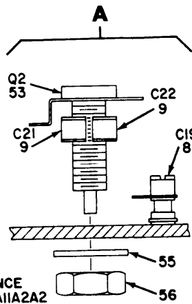
Figure 18. Power Oscillator Assembly (A11A2A2) (Sheet 1 of 2)
