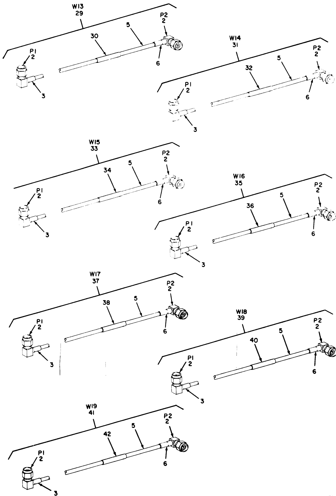
Figure 27. Cable Assemblies, RF (152177-- and 151178--) (Sheet 3 of 4)
