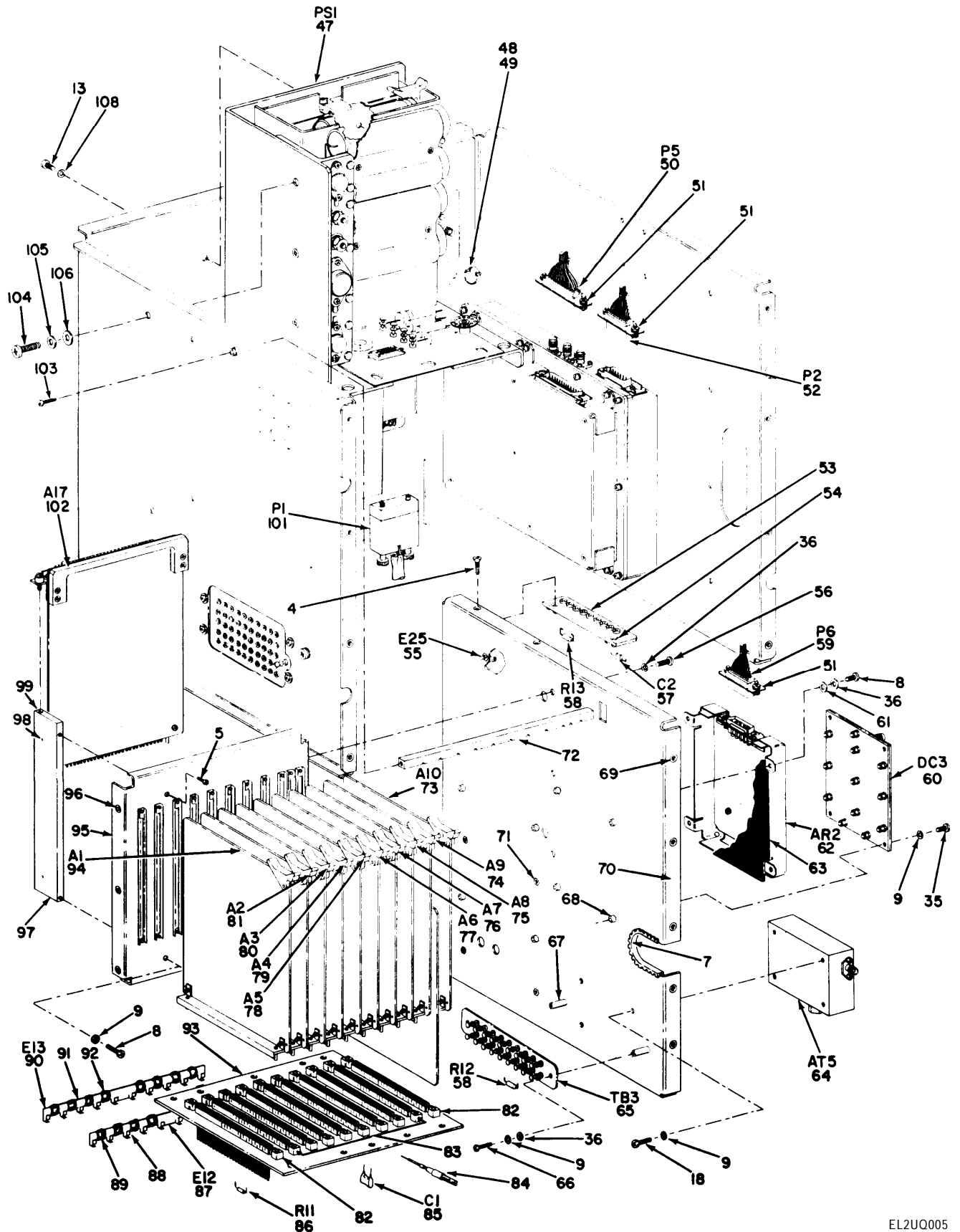
Figure 2. Test Set, Radar TS-3394A/TPM-25 (Sheet 3 of 4)
