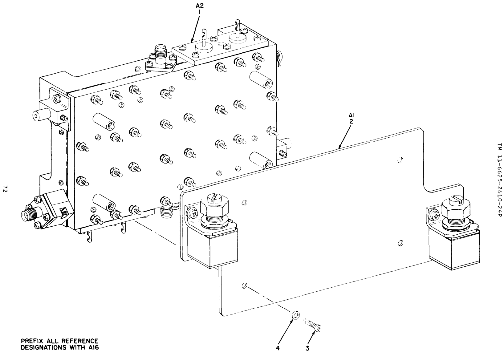
Figure 20. Modulator, Dual Signal Generator (A16)
