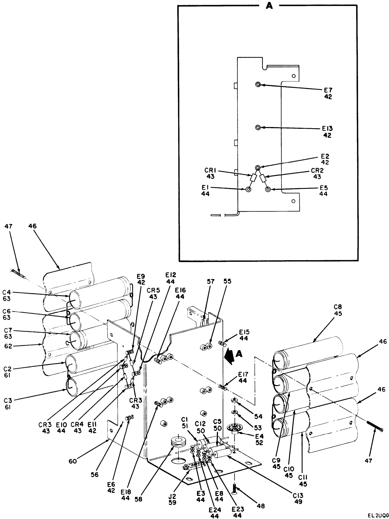
Figure 23. Power Supply Assembly (PS1)(Sheet 2 of 2)
