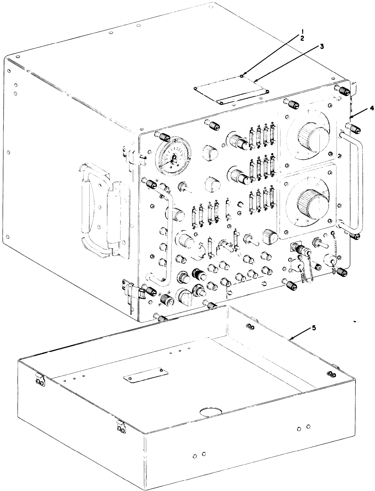
Figure 1. Radar Test Set AN/TPM-25A (Sheet 1 of 2)
