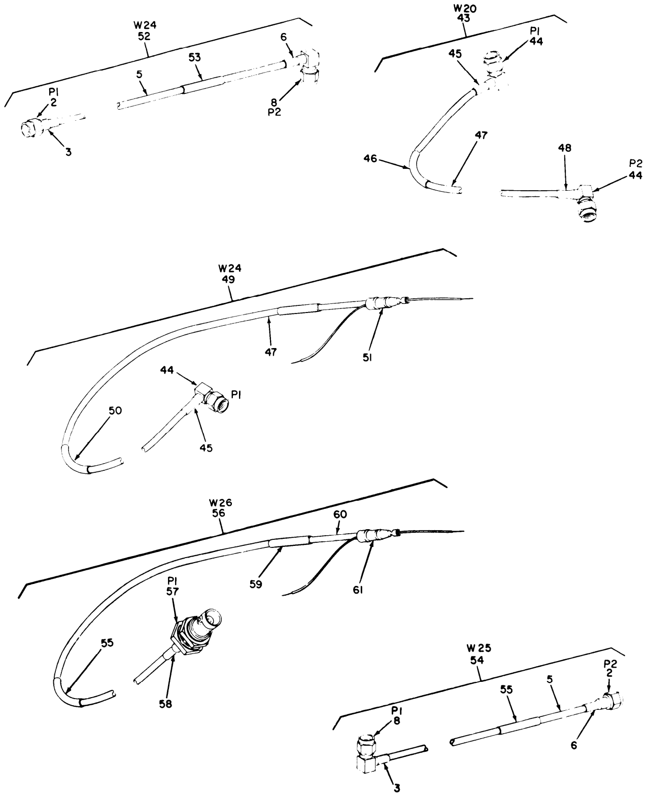
Figure 27. Cable Assemblies, RF (152177-- and 151178--) (Sheet 4 of 4)
