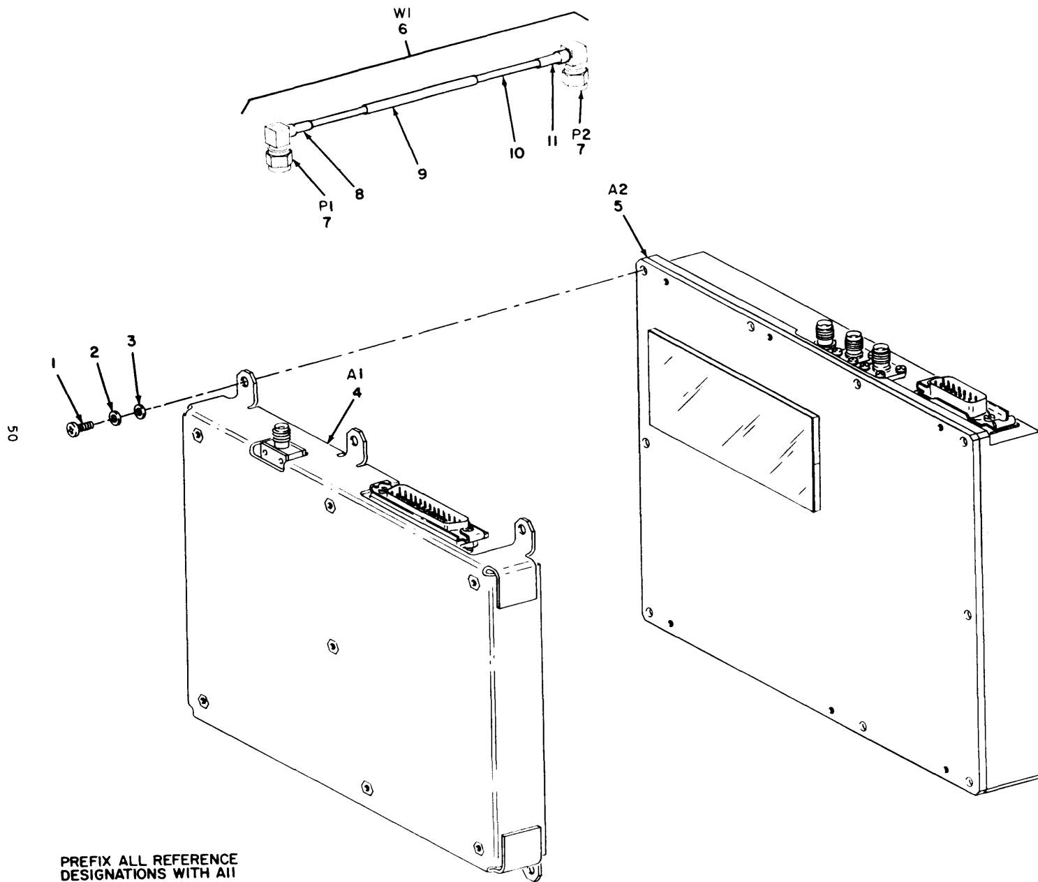
Figure 14. RF Generator Assembly (A11)
