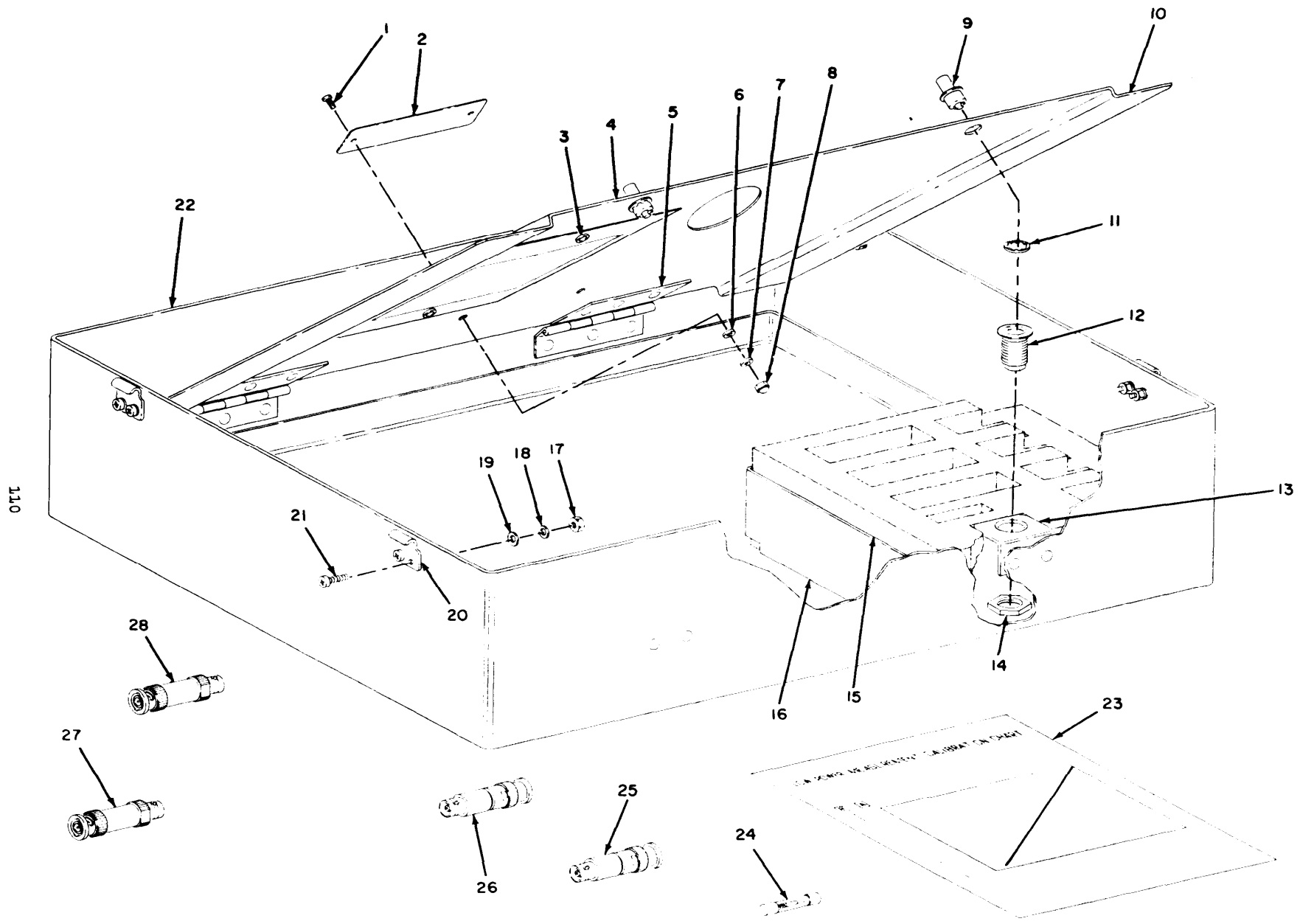
Figure 29. Cover, Test Set MX-9929/TPM-25A
