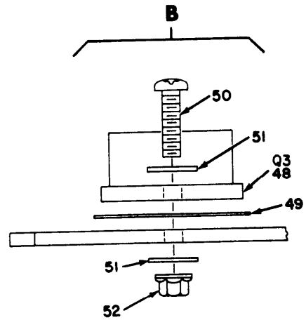
Figure 18. Power Oscillator Assembly (A11A2A2) (Sheet 1 of 2)
