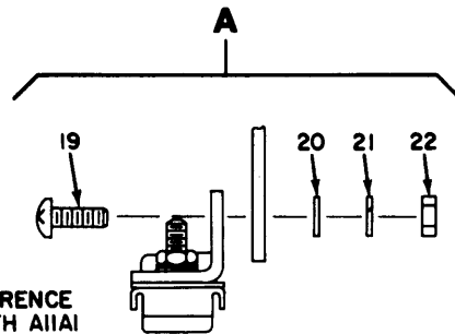
Figure 15. Marker/Ramp Generator Assembly (A11A1) (Sheet 1 of 2)
